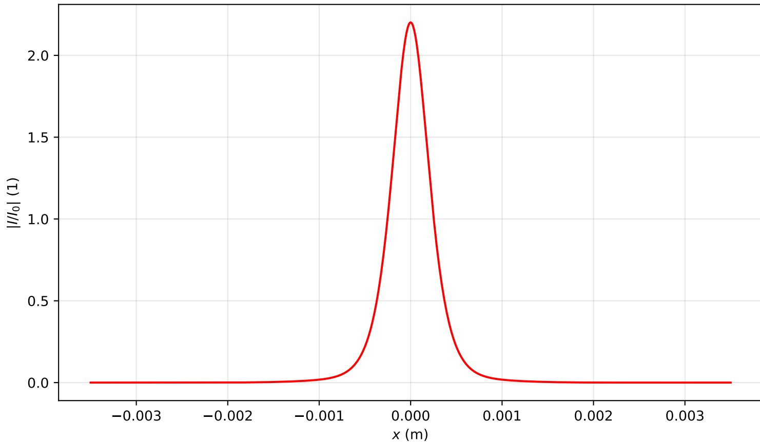
Intensity profile I(x, y = 0, z = 2.149)/I_0 , \text{Pin}=1.0\text{Pcr} , artificial time
